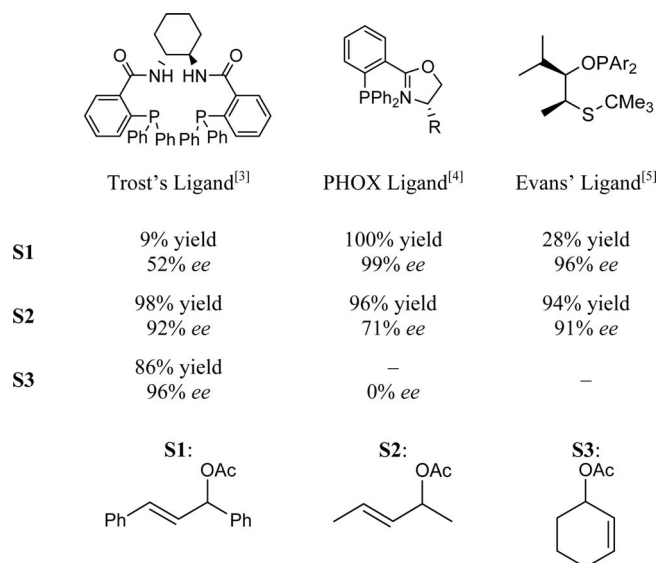
Figure 2. Overview of the best results obtained for some of the most popular ligands in the asymmetric allylic alkylations of S1 – S3 .
