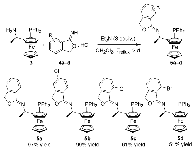
Scheme 1. Synthesis of imidate-phosphane ligands 5a–d .
