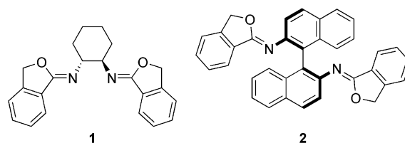
Figure 1. C 2 -symmetrical imidate ligands.
